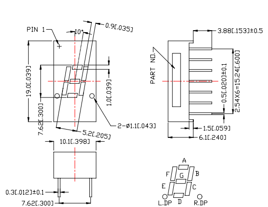
B . WCN1-XX30XX-A56T/C56T
