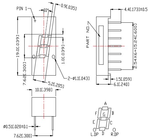
A . WCN1-XX30XX-A21T/C21T
